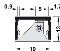
LED 5 mm
